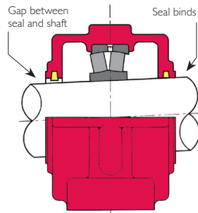
DOUBLE ROW SPHERICAL BEARING
