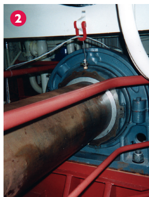
2. A typical installation of a Cooper BCP on a propulsion shafting application.
