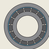
High-capacity bearing with outer ring centred cage
